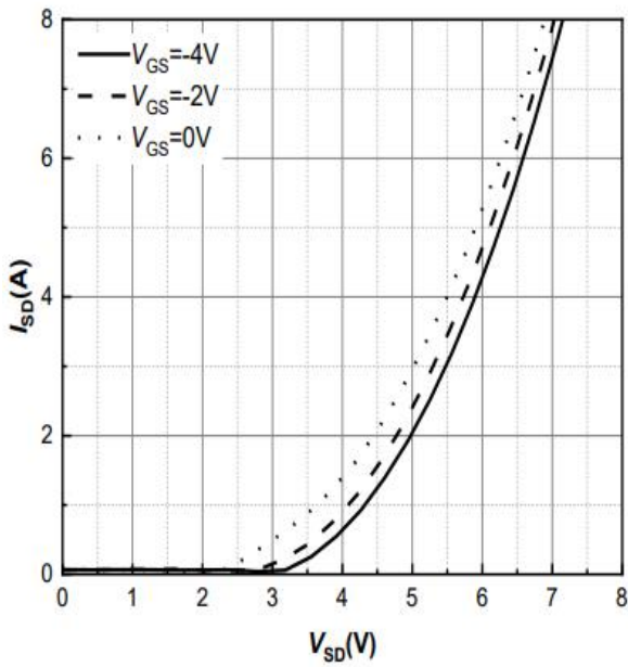
Figure 9. Body Diode Characteristic T_j=25^{\circ}\text{C}
