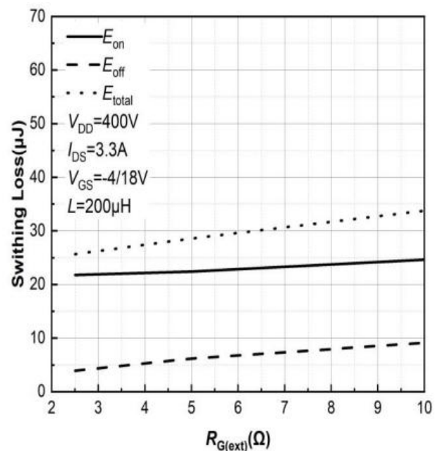
Figure 24. Clamped Inductive Switching Energy vs. R_{G(ext)} T_j=175^\circ\text{C}
