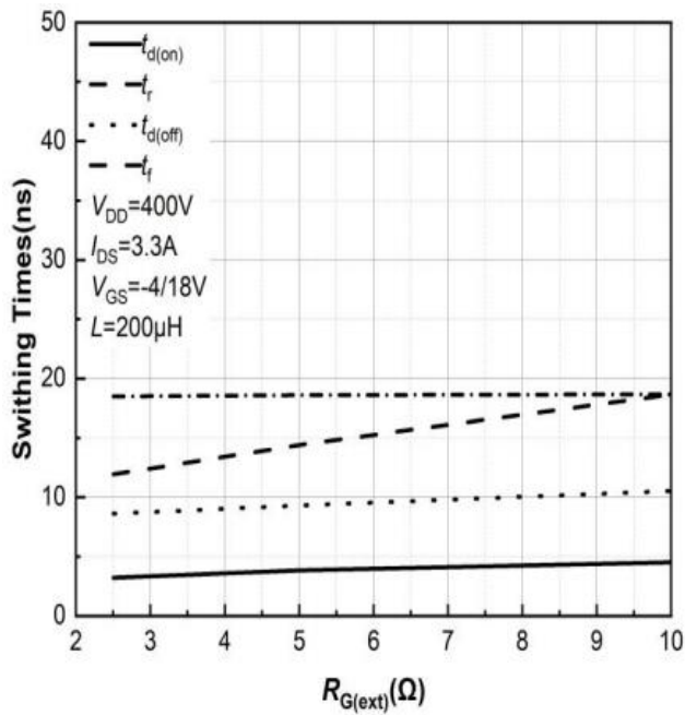
Figure 25. Switching Times vs. R_{G(ext)} T_J = 25^\circ\text{C}
