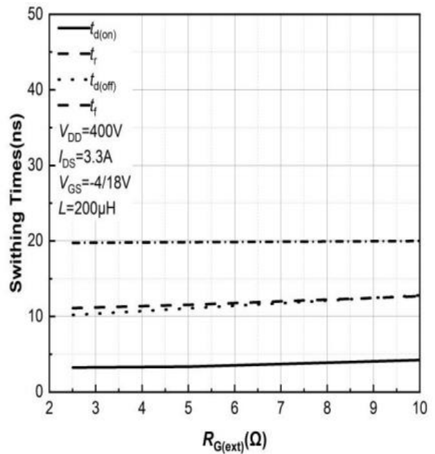
Figure 26. Switching Times vs. R_{G(ext)} T_J = 175^\circ\text{C}
