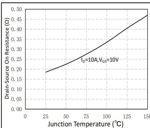
Fig5. R_{DS(on)} vs T_J
