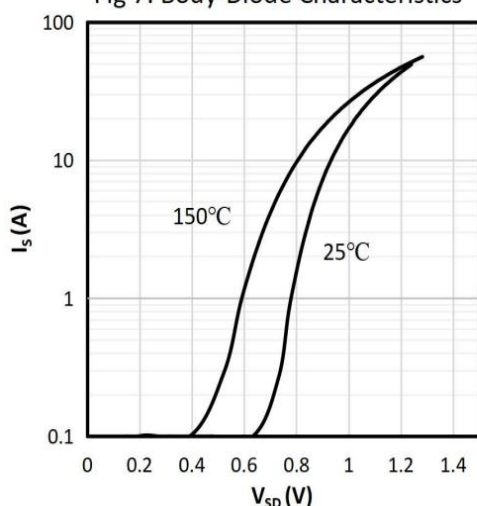
Fig 7: Body-Diode Characteristics
