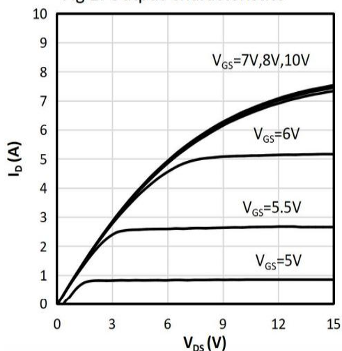
Fig 1: Output Characteristics
