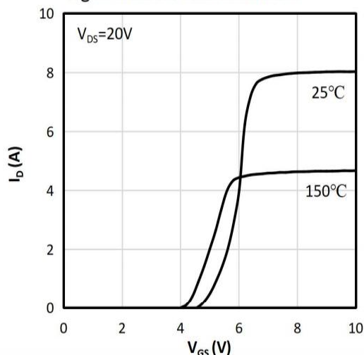
Fig 2: Transfer Characteristics
