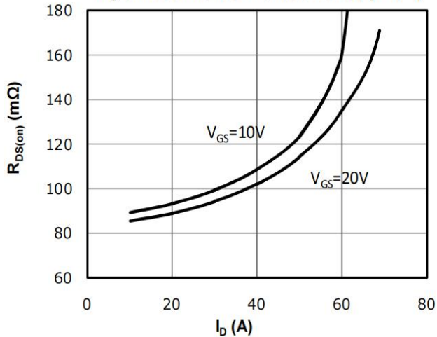
Fig 5: R_{DS(on)} Vs I_{DS} Characteristics (Tj=25°C)
