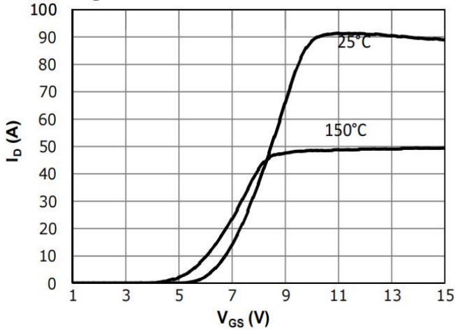
Fig 3: Transfer Characteristics
