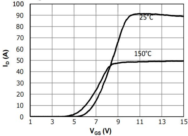
Fig 3: Transfer Characteristics
