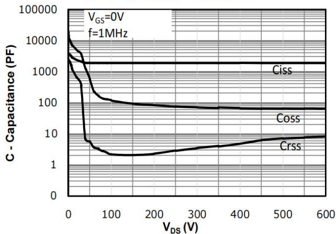
Fig 11: Capacitance Characteristics
