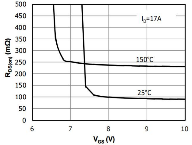
Fig 8: Rds(on) vs Gate Voltage
