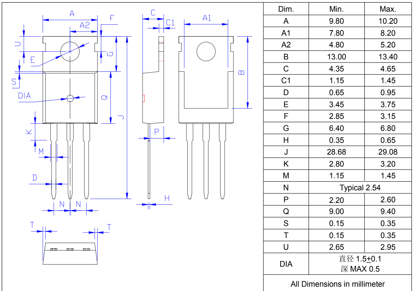
TO-220C 封装尺寸 Package size
