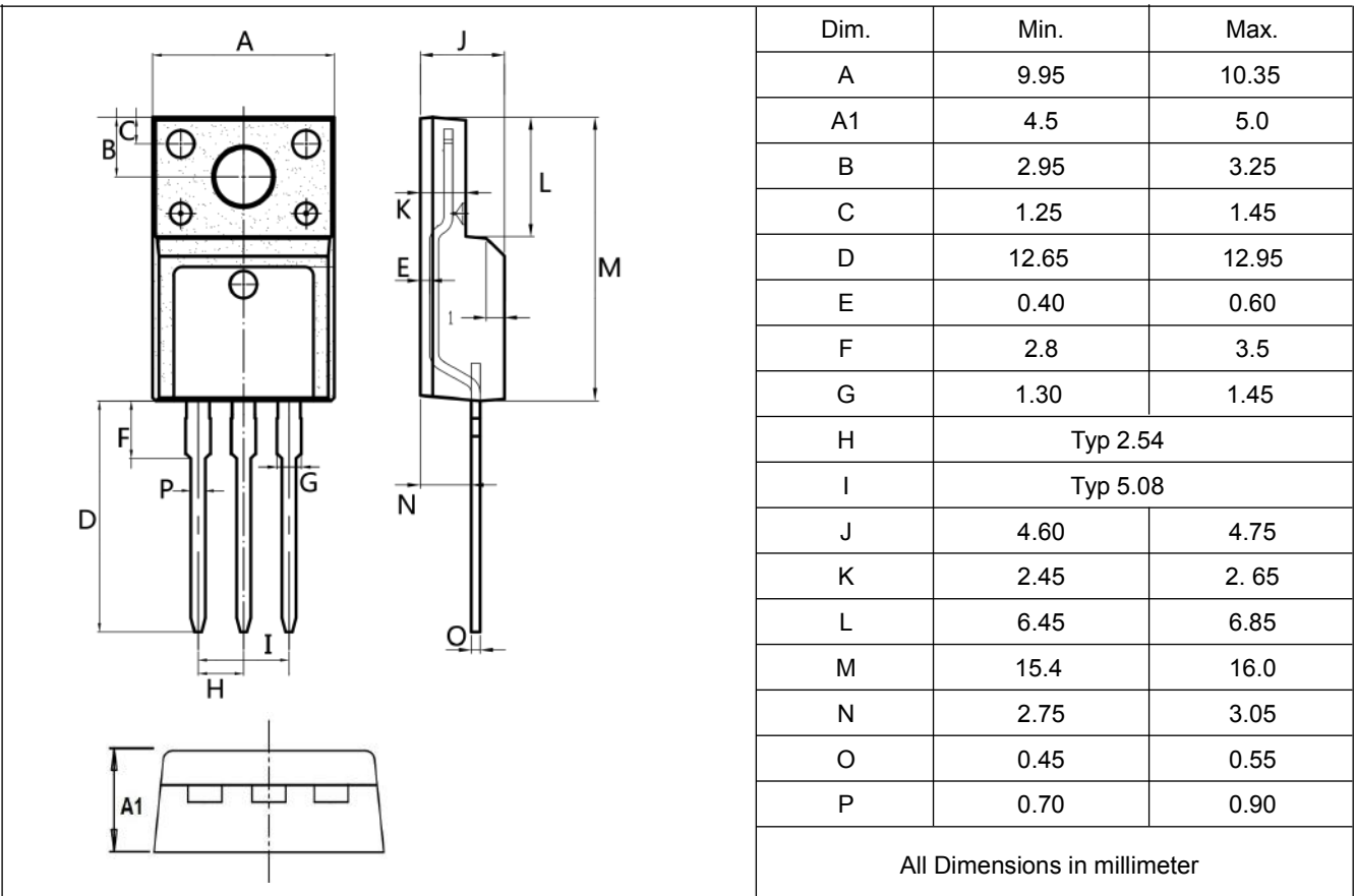
TO-220F 封装尺寸 Package size
