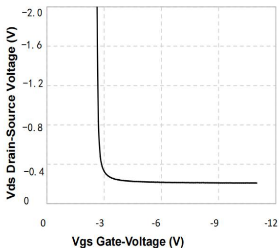
Figure 7. Breakdown Voltage Variation vs Gate-Voltage
