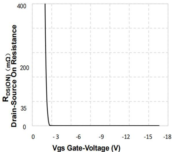
Figure 8. On-Resistance Variation vs Gate Voltage
