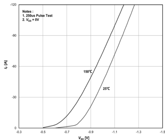
Figure 4. Body Diode Forward Voltage Variation with Current
