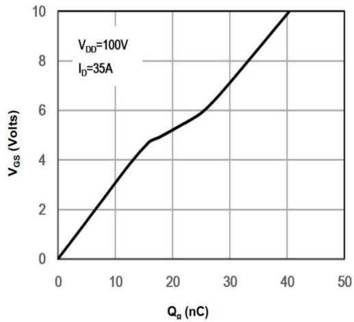
Figure 7: Gate-Charge Characteristics
