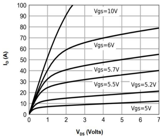
Figure 1: On-Region Characteristics
