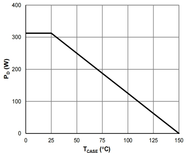
Figure 10: Power De-rating
