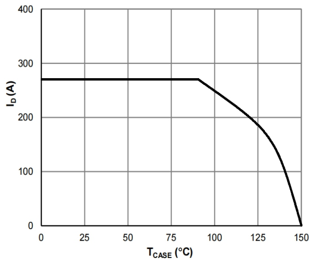
Figure 9: Current De-rating
