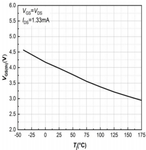
Figure 11. Threshold Voltage vs. Temperature
