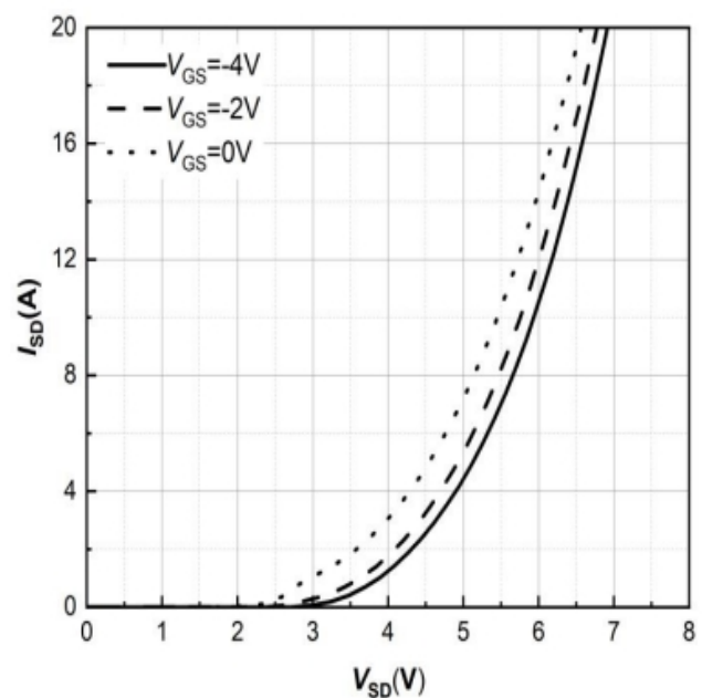
Figure 8. Body Diode Characteristic T_J = -40°C
