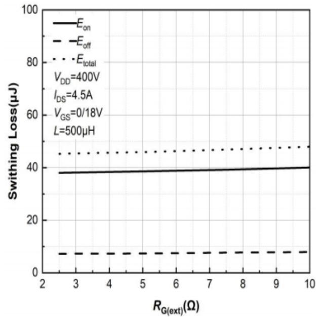
Figure 24. Clamped Inductive Switching Energy vs. R_{G(\text{ext})} T_j=175^{\circ}\text{C}
