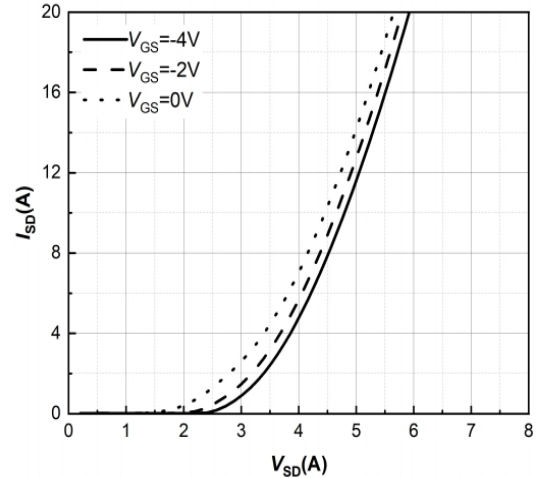
Figure 8. Body Diode Characteristic T_J = -40^\circ\text{C}
