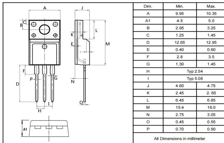
TO-220F
